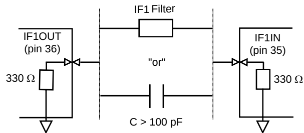
Figure 14. Schematic Input of IF1 Amplifier
